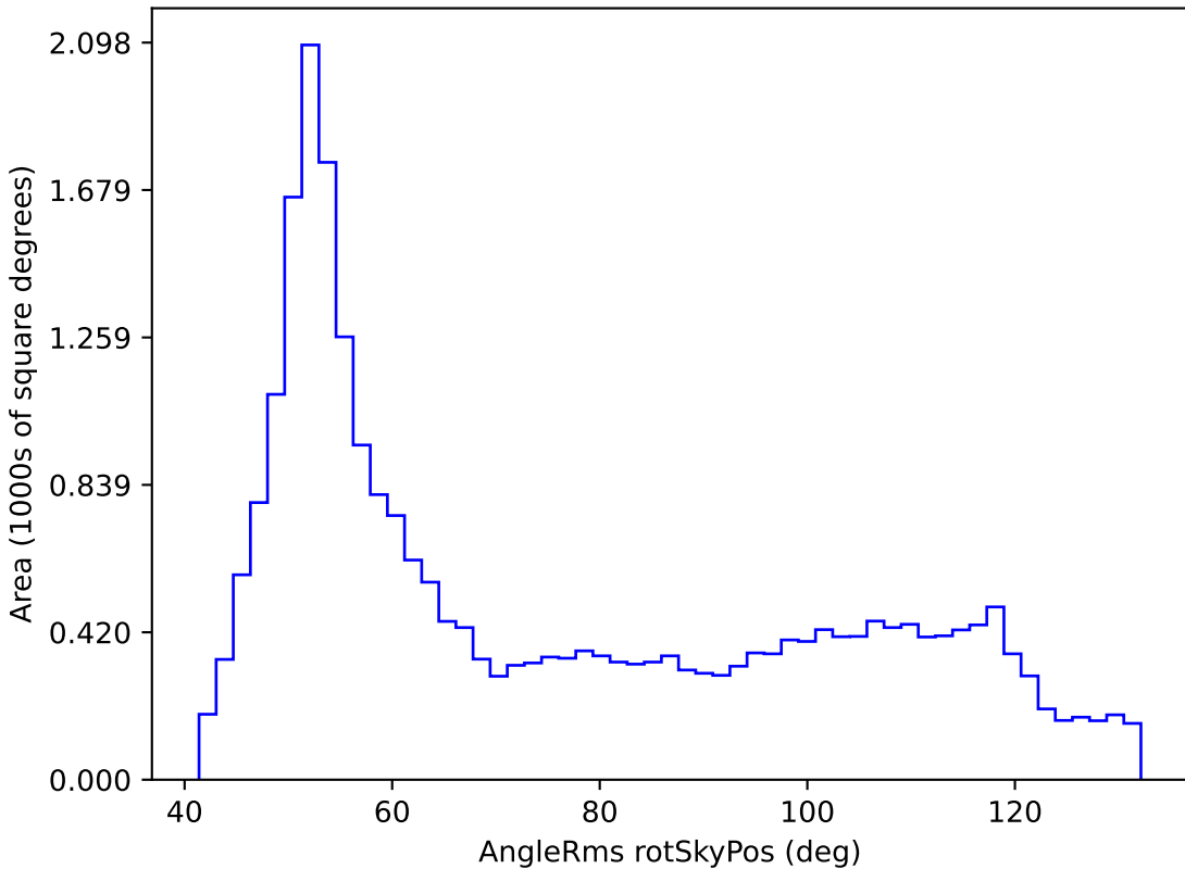
baseline_v2.1_10yrs All sky all bands: AngleRms rotSkyPos
