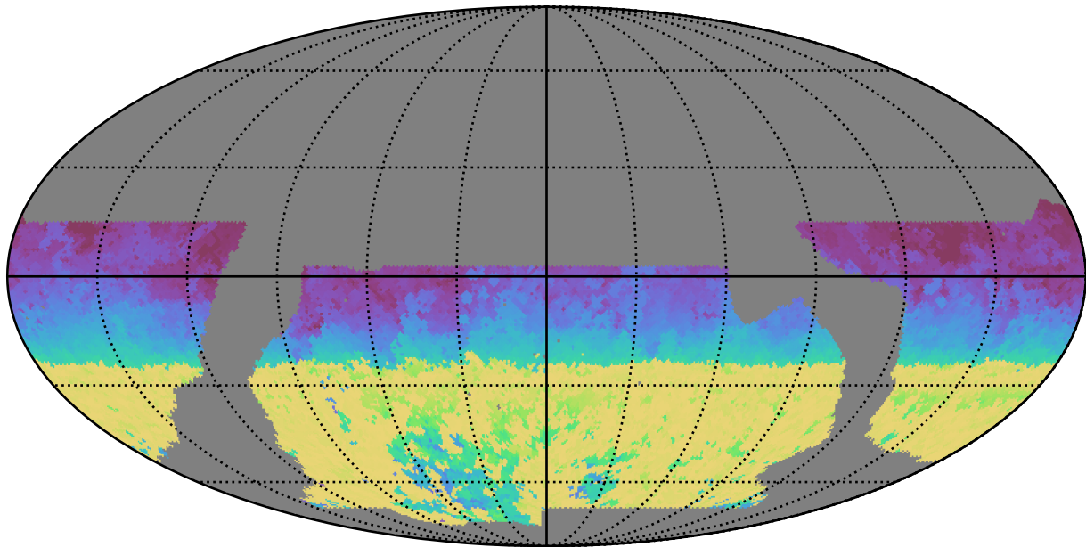
baseline_v2.1_10yrs WFD z band: AngleRange rotSkyPos
