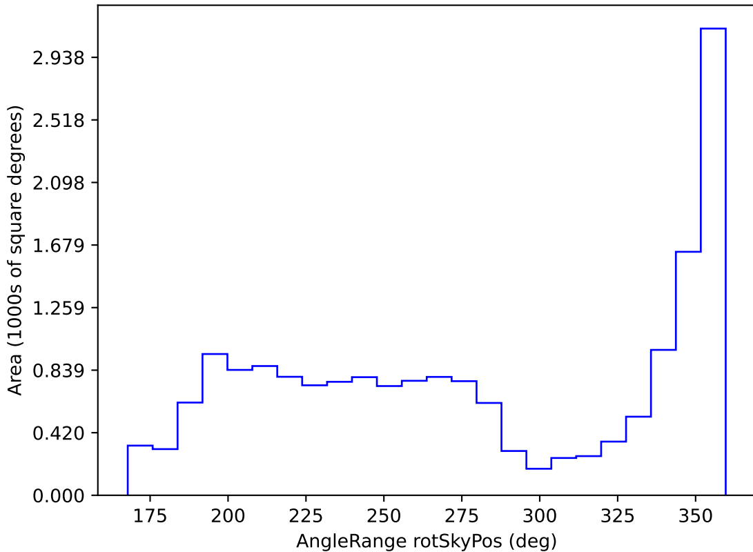
baseline_v2.1_10yrs WFD u band: AngleRange rotSkyPos
