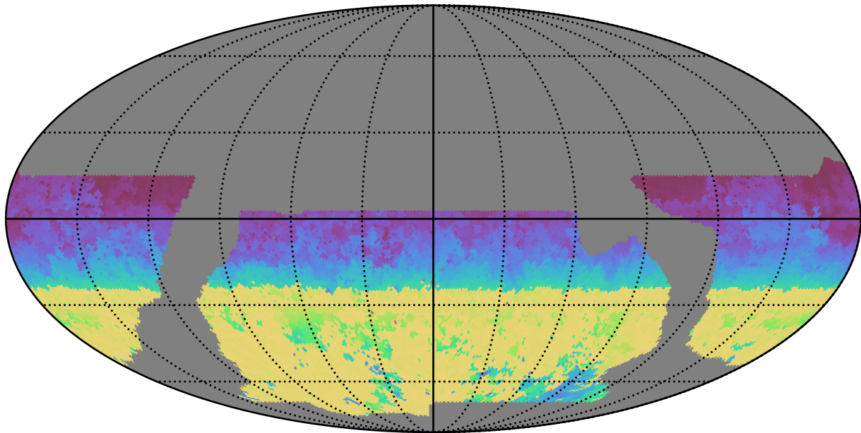
baseline_v2.1_10yrs WFD r band: AngleRange rotSkyPos
