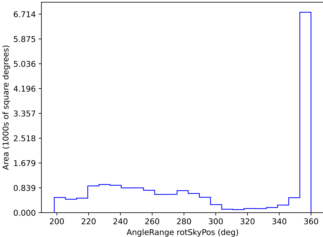
baseline_v2.1_10yrs WFD r band: AngleRange rotSkyPos
