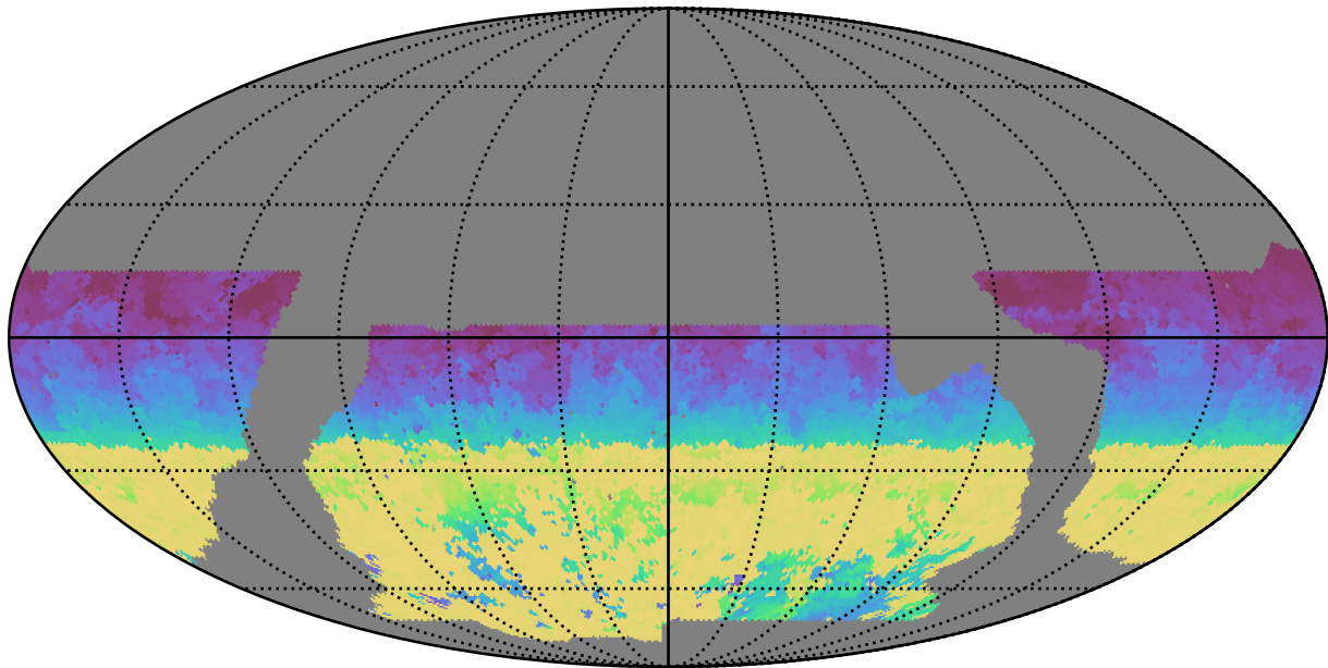
baseline_v2.1_10yrs WFD i band: AngleRange rotSkyPos
