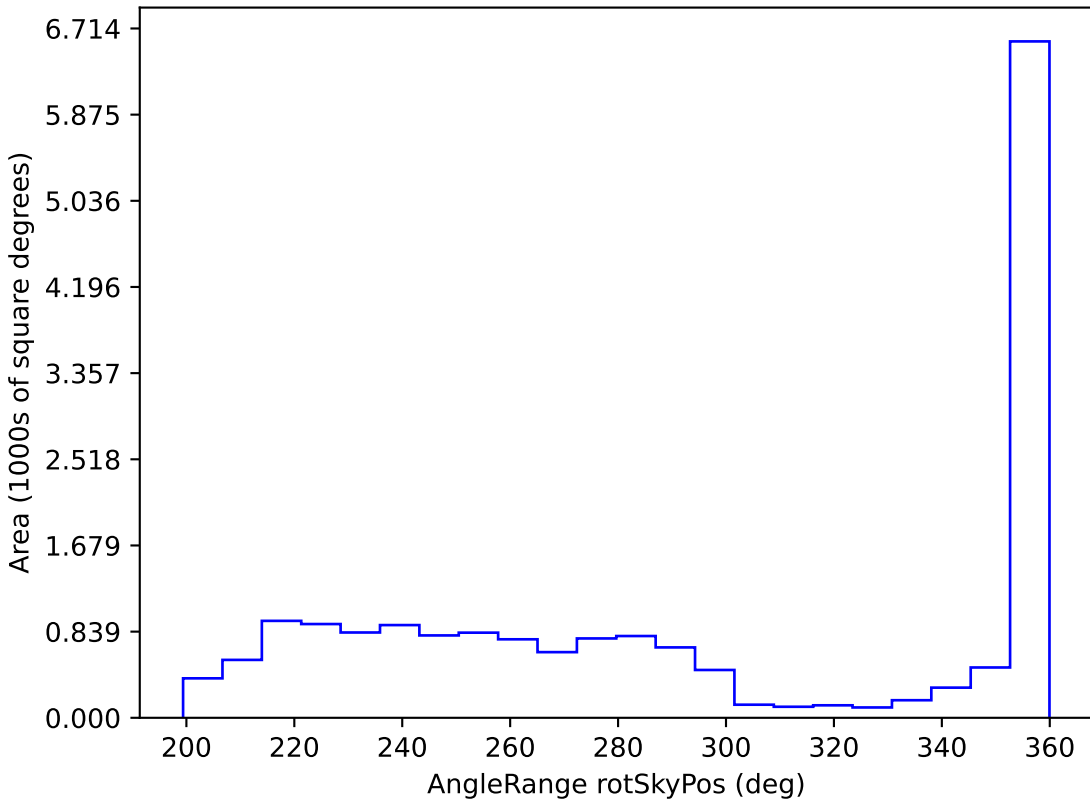
baseline_v2.1_10yrs WFD i band: AngleRange rotSkyPos
