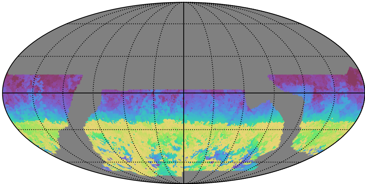
baseline_v2.1_10yrs WFD g band: AngleRange rotSkyPos
