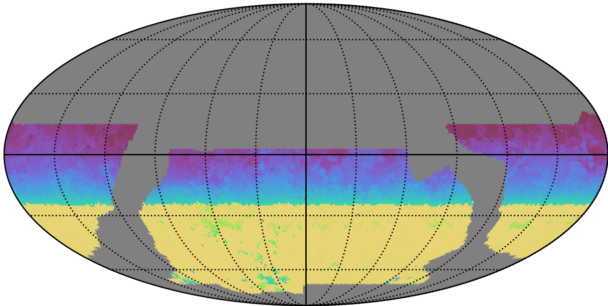
baseline_v2.1_10yrs WFD all bands: AngleRange rotSkyPos
