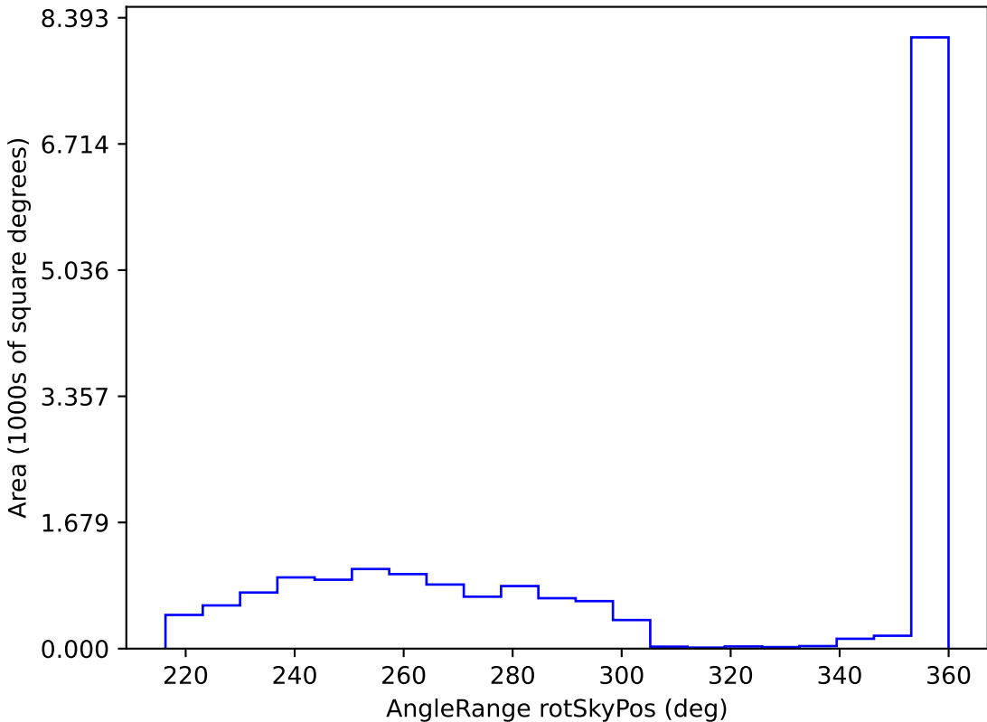
baseline_v2.1_10yrs WFD all bands: AngleRange rotSkyPos
