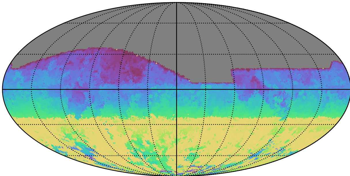
baseline_v2.1_10yrs All sky z band: AngleRange rotSkyPos
