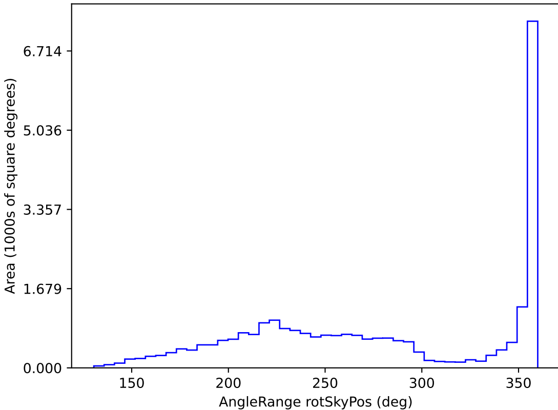
baseline_v2.1_10yrs All sky z band: AngleRange rotSkyPos
