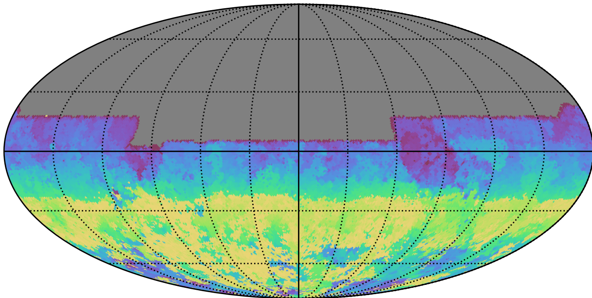
baseline_v2.1_10yrs All sky u band: AngleRange rotSkyPos
