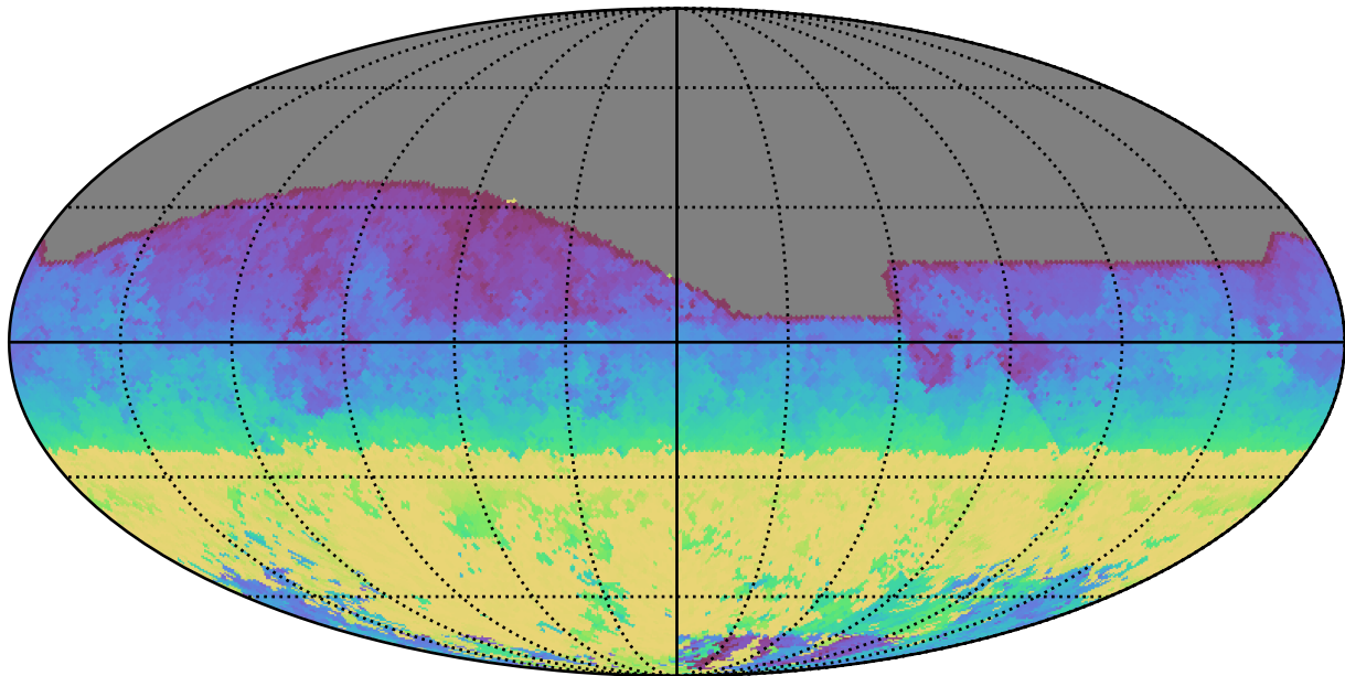
baseline_v2.1_10yrs All sky r band: AngleRange rotSkyPos
