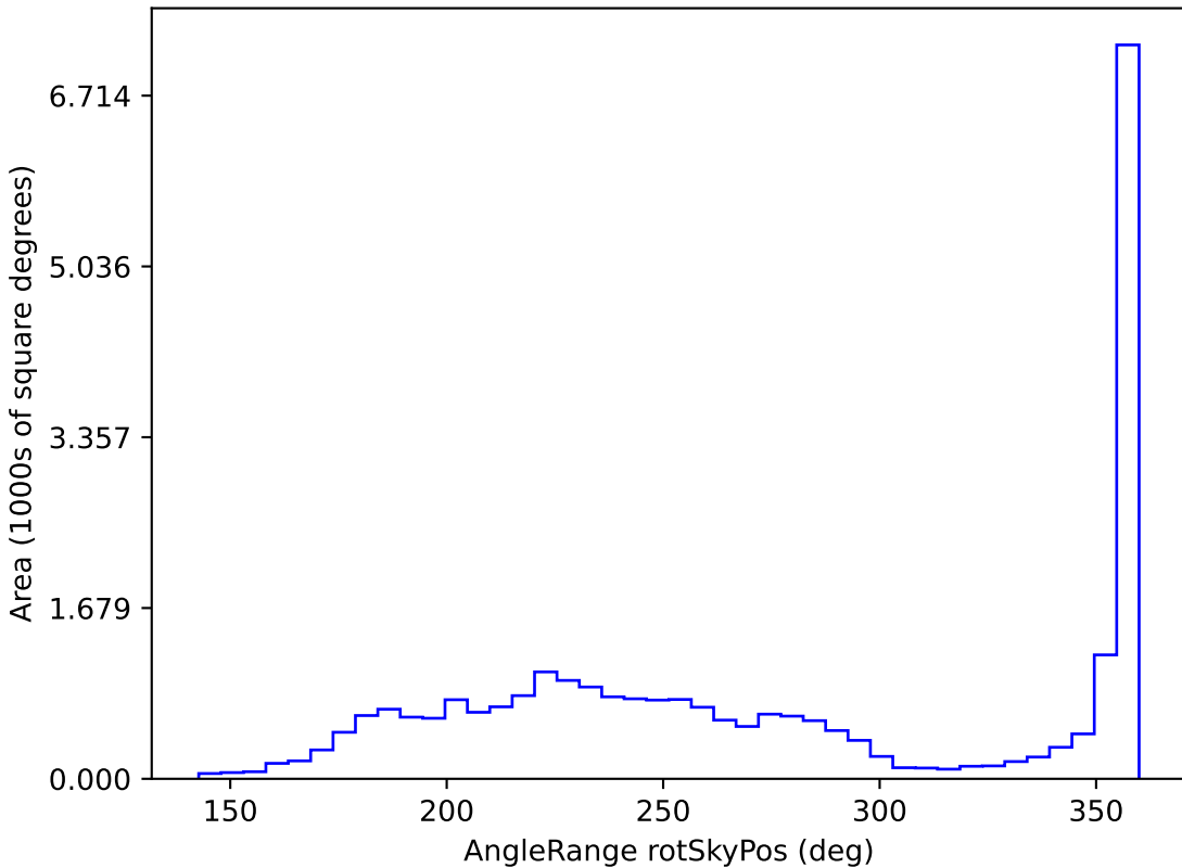
baseline_v2.1_10yrs All sky r band: AngleRange rotSkyPos
