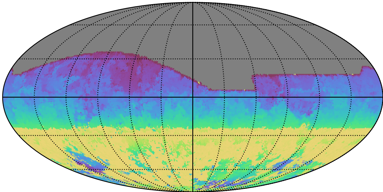
baseline_v2.1_10yrs All sky i band: AngleRange rotSkyPos
