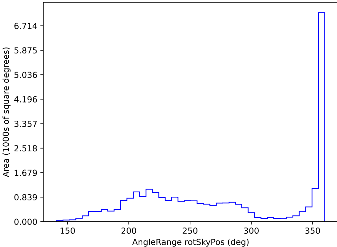
baseline_v2.1_10yrs All sky i band: AngleRange rotSkyPos
