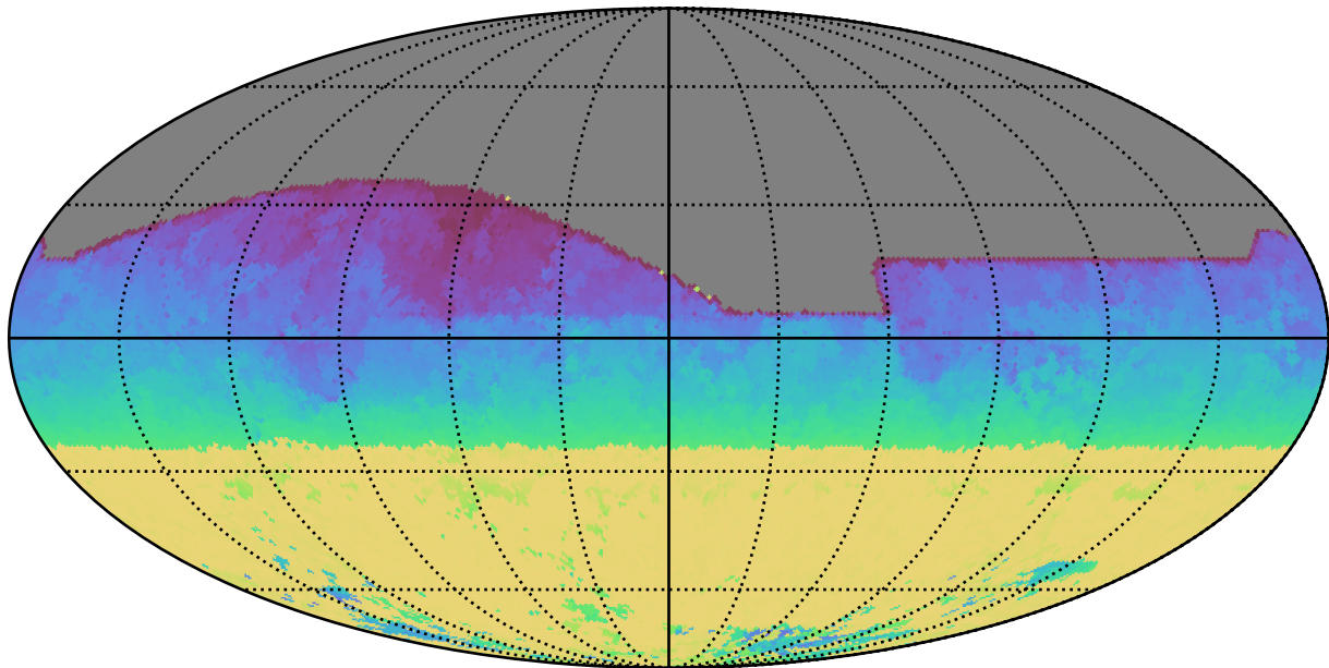
baseline_v2.1_10yrs All sky all bands: AngleRange rotSkyPos
