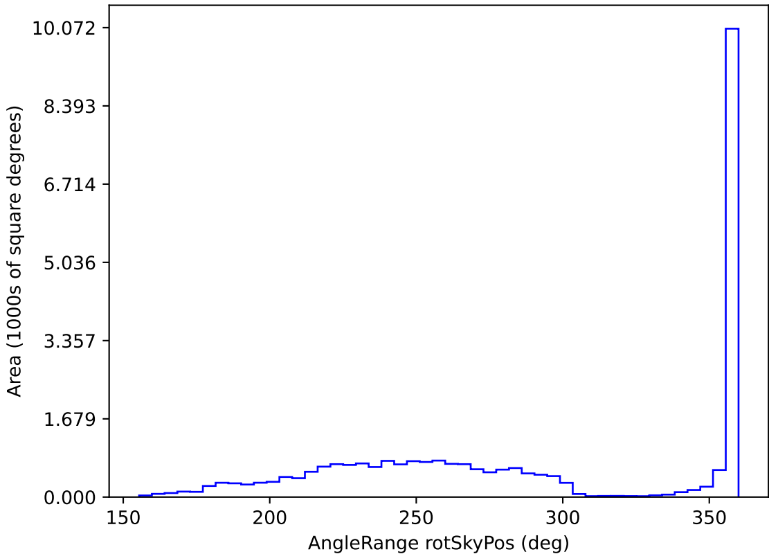
baseline_v2.1_10yrs All sky all bands: AngleRange rotSkyPos
