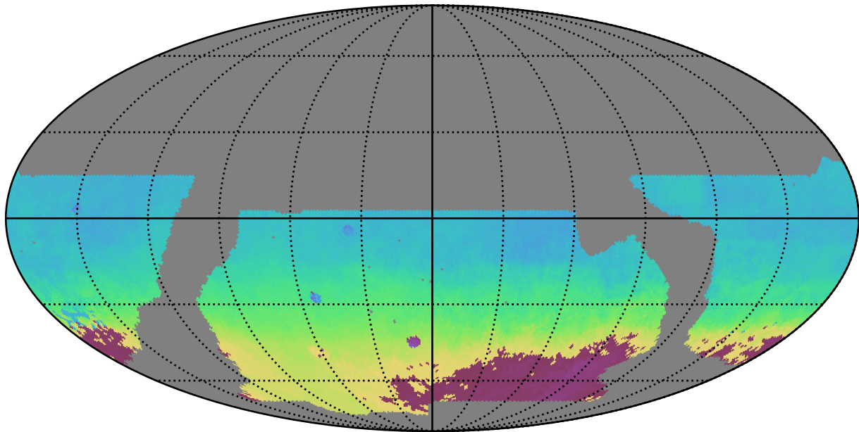
baseline_v2.1_10yrs WFD z band: AngleMean rotSkyPos
