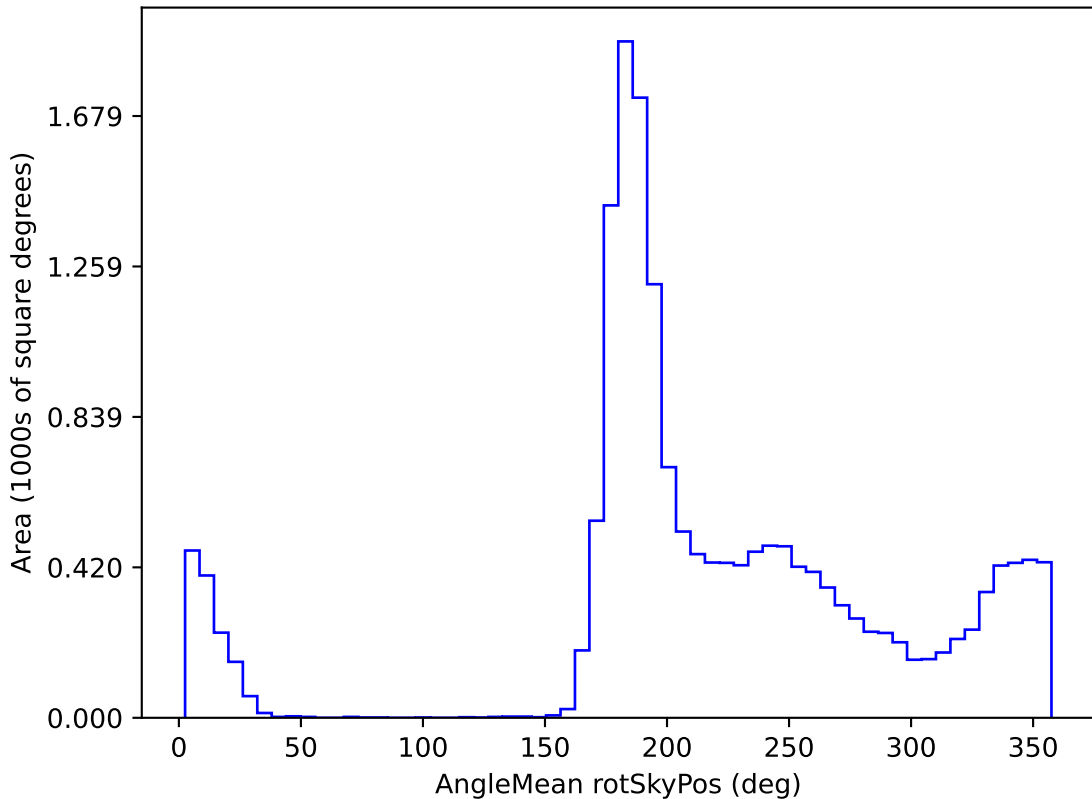
baseline_v2.1_10yrs WFD z band: AngleMean rotSkyPos
