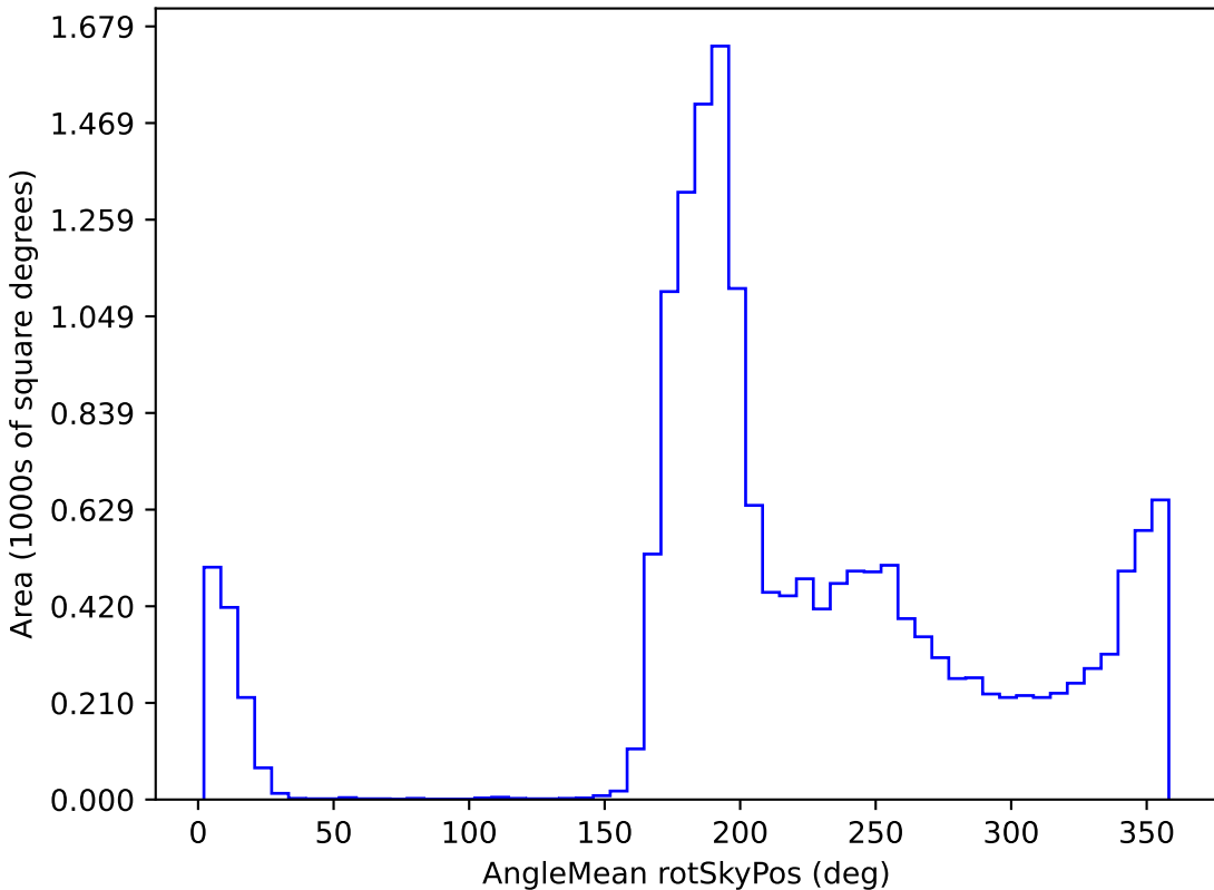
baseline_v2.1_10yrs WFD y band: AngleMean rotSkyPos
