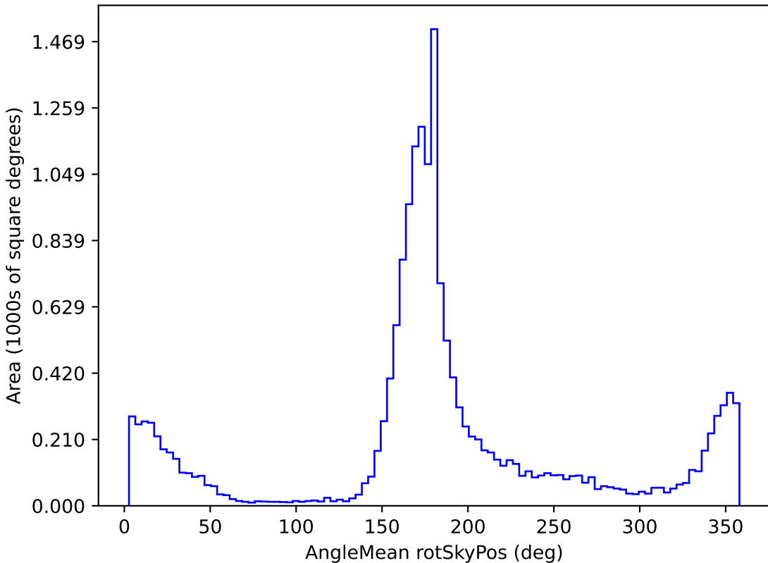
baseline_v2.1_10yrs WFD u band: AngleMean rotSkyPos
