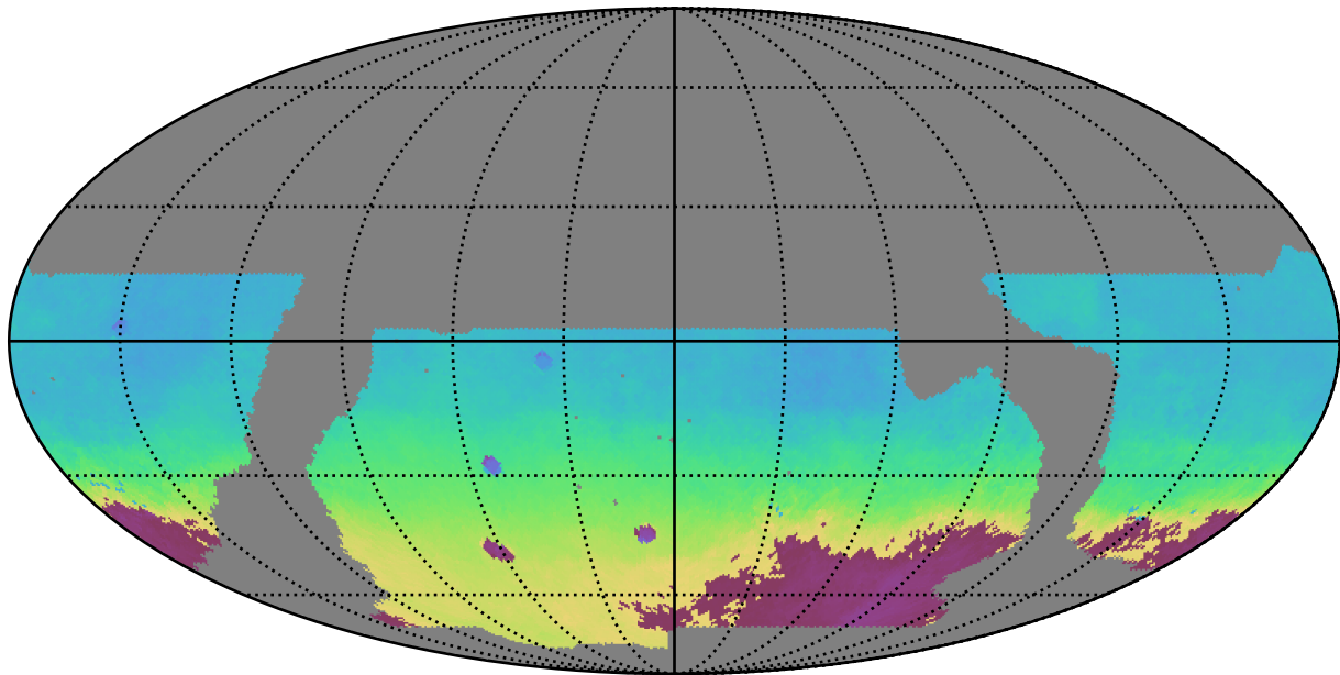
baseline_v2.1_10yrs WFD i band: AngleMean rotSkyPos
