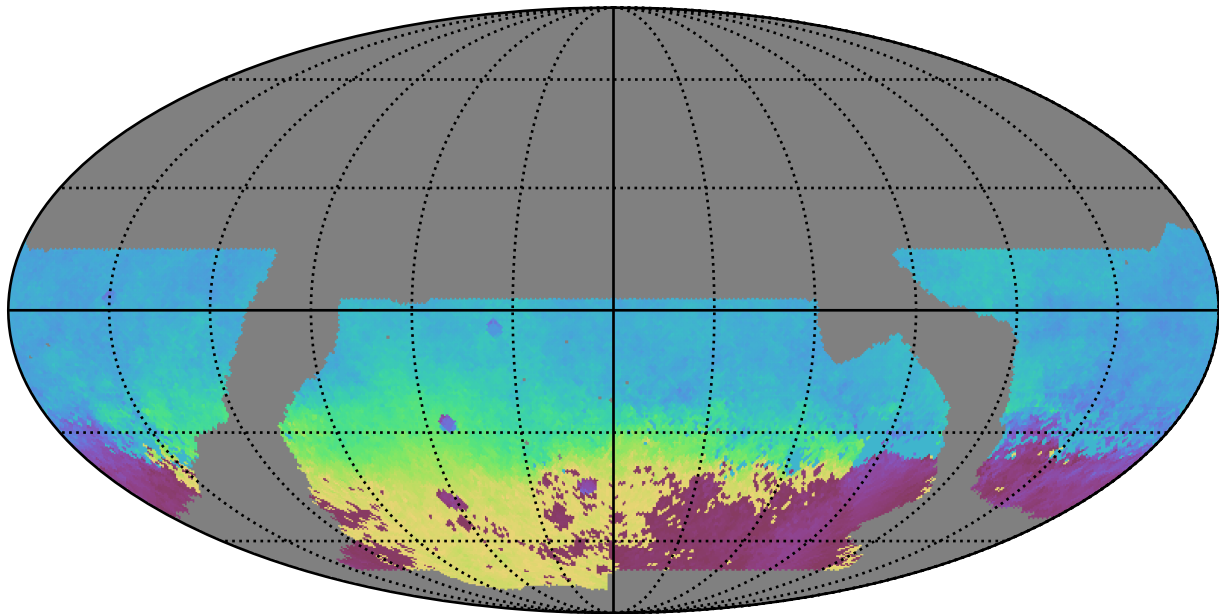
baseline_v2.1_10yrs WFD g band: AngleMean rotSkyPos
