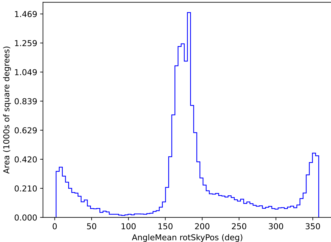
baseline_v2.1_10yrs WFD g band: AngleMean rotSkyPos
