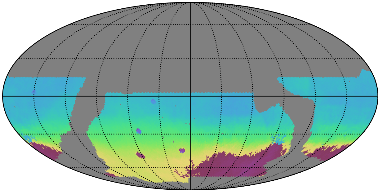
baseline_v2.1_10yrs WFD all bands: AngleMean rotSkyPos
