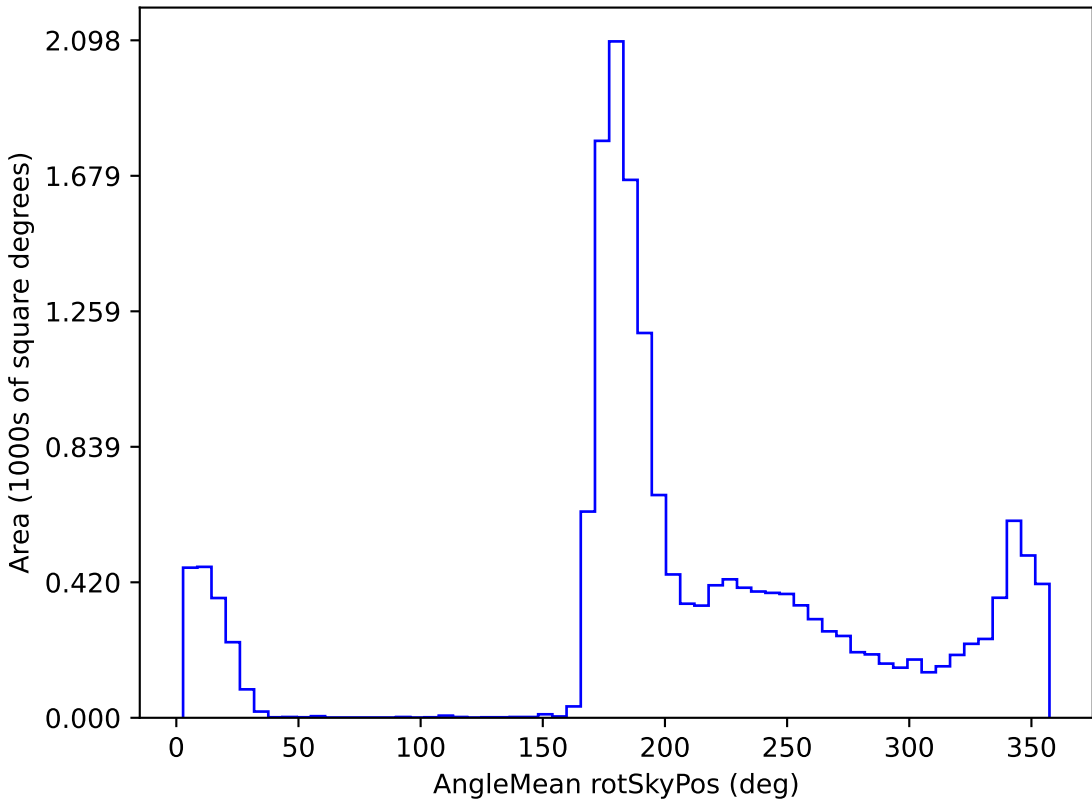
baseline_v2.1_10yrs WFD all bands: AngleMean rotSkyPos
