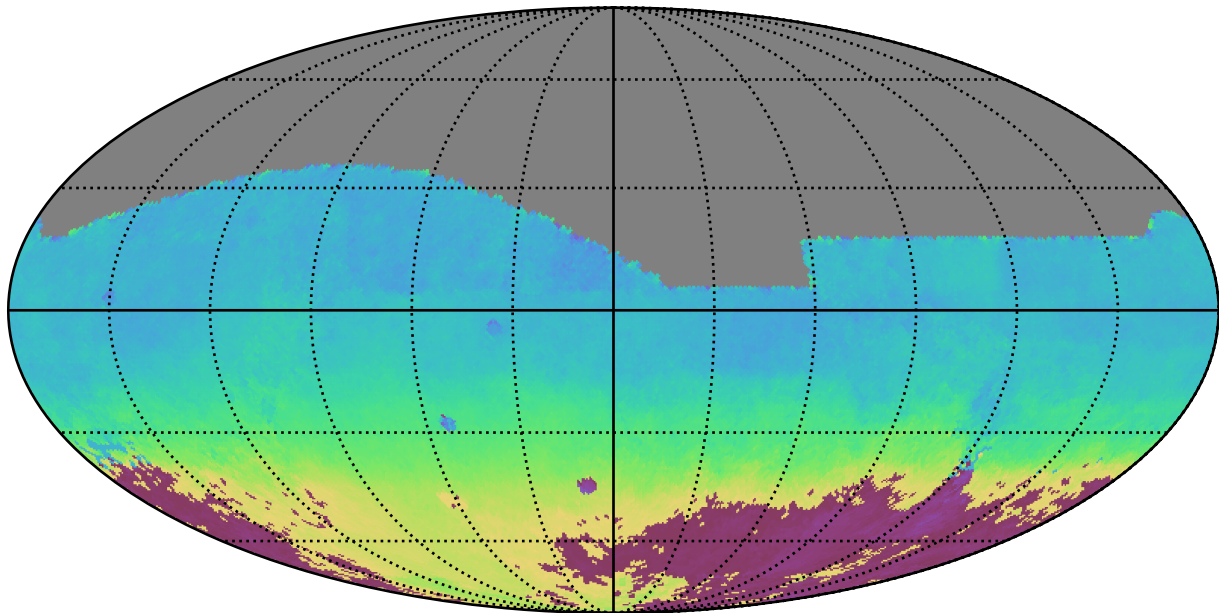
baseline_v2.1_10yrs All sky z band: AngleMean rotSkyPos
