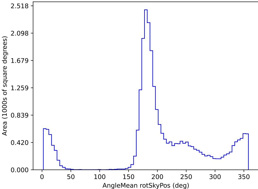
baseline_v2.1_10yrs All sky z band: AngleMean rotSkyPos
