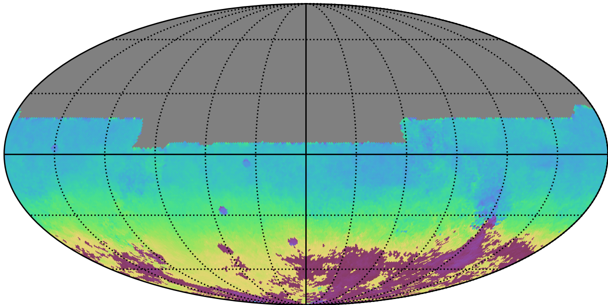
baseline_v2.1_10yrs All sky y band: AngleMean rotSkyPos
