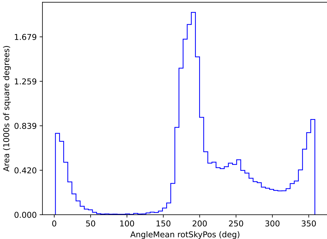
baseline_v2.1_10yrs All sky y band: AngleMean rotSkyPos
