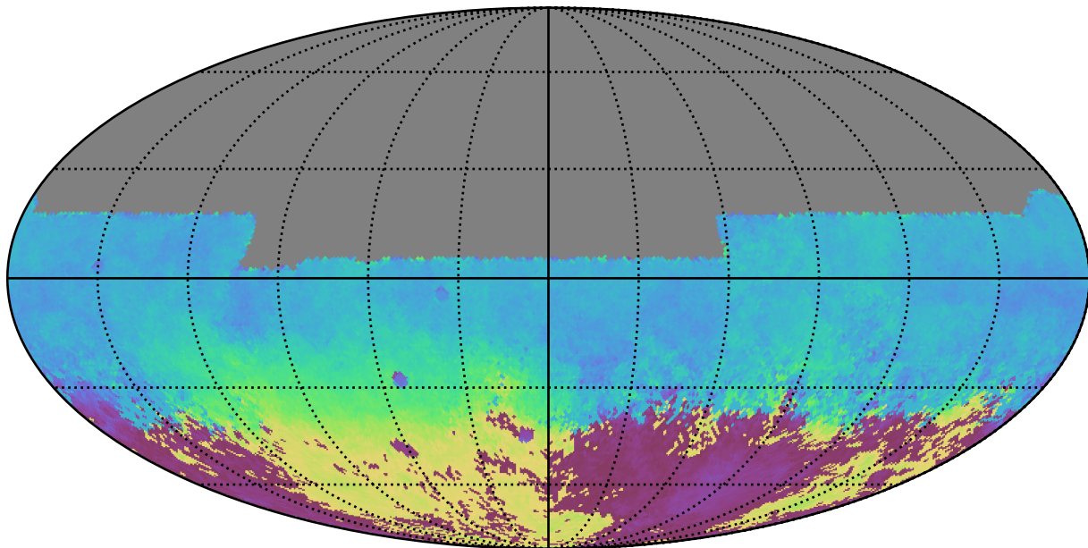
baseline_v2.1_10yrs All sky u band: AngleMean rotSkyPos
