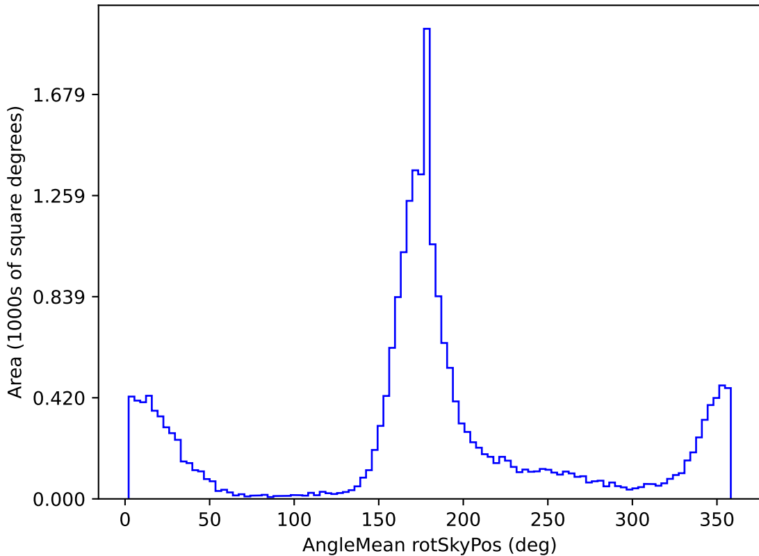
baseline_v2.1_10yrs All sky u band: AngleMean rotSkyPos
