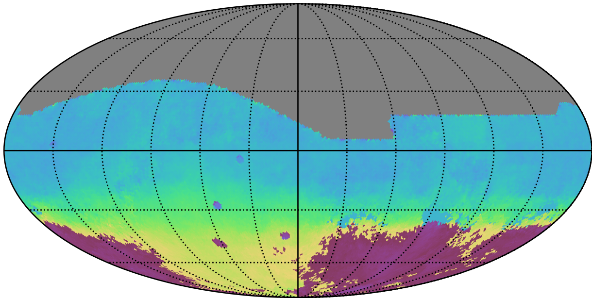
baseline_v2.1_10yrs All sky r band: AngleMean rotSkyPos
