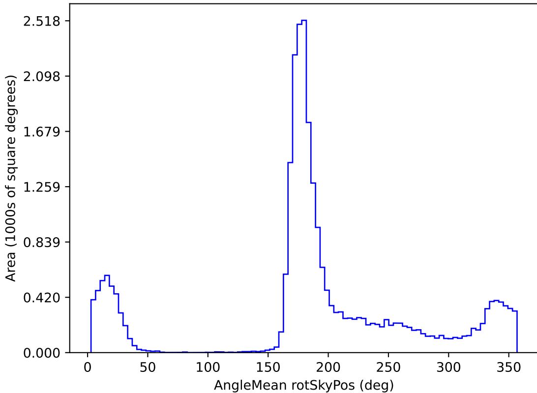
baseline_v2.1_10yrs All sky r band: AngleMean rotSkyPos
