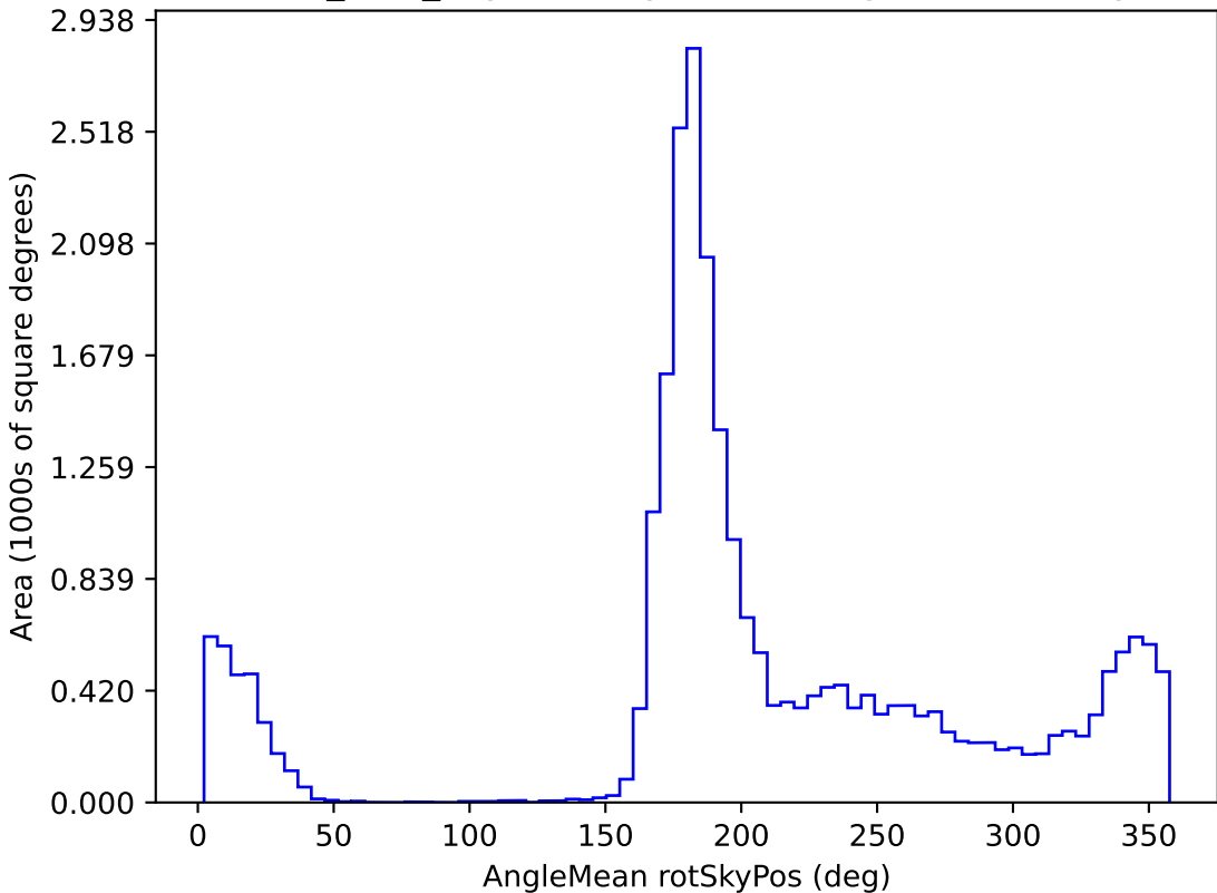
baseline_v2.1_10yrs All sky i band: AngleMean rotSkyPos
