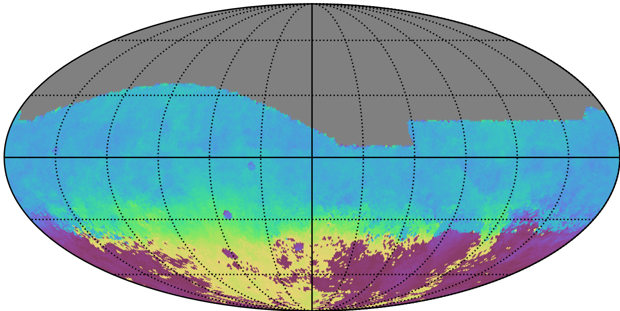
baseline_v2.1_10yrs All sky g band: AngleMean rotSkyPos
