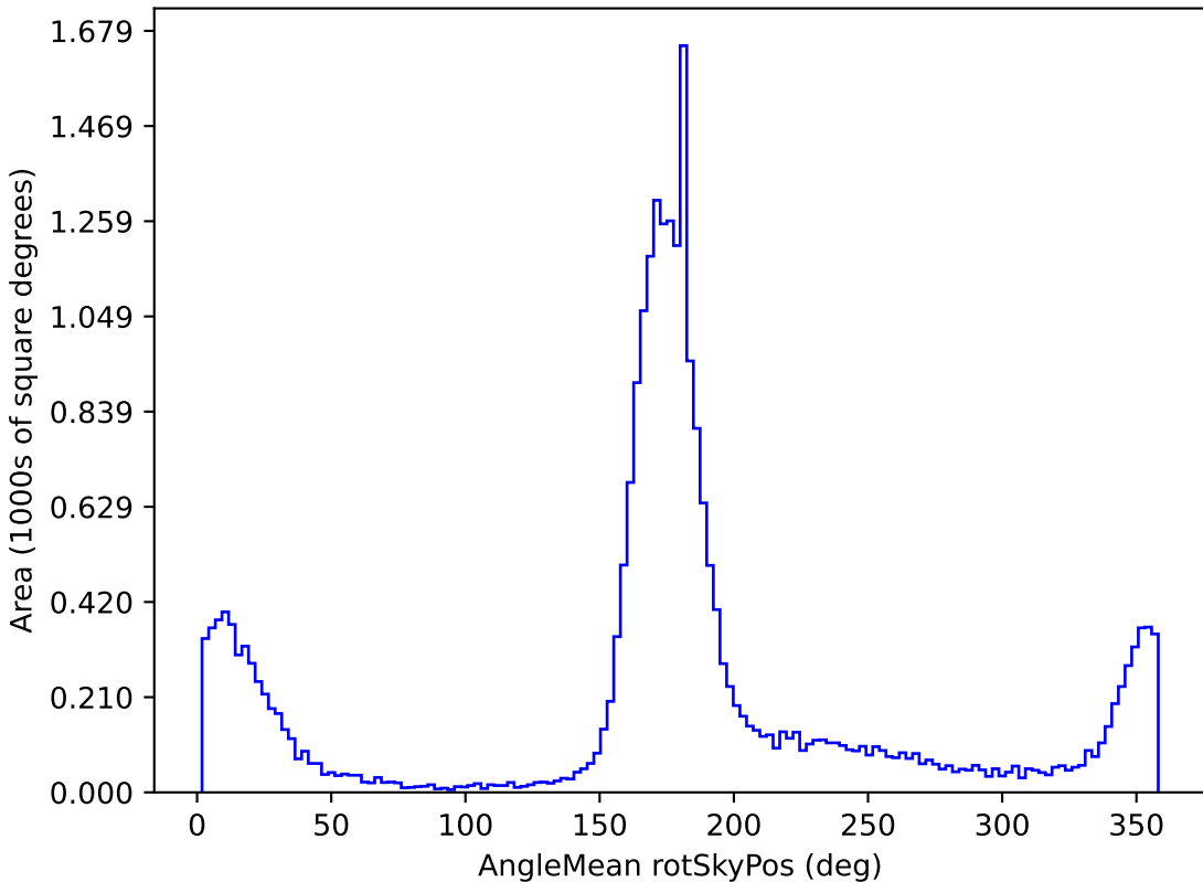
baseline_v2.1_10yrs All sky g band: AngleMean rotSkyPos
