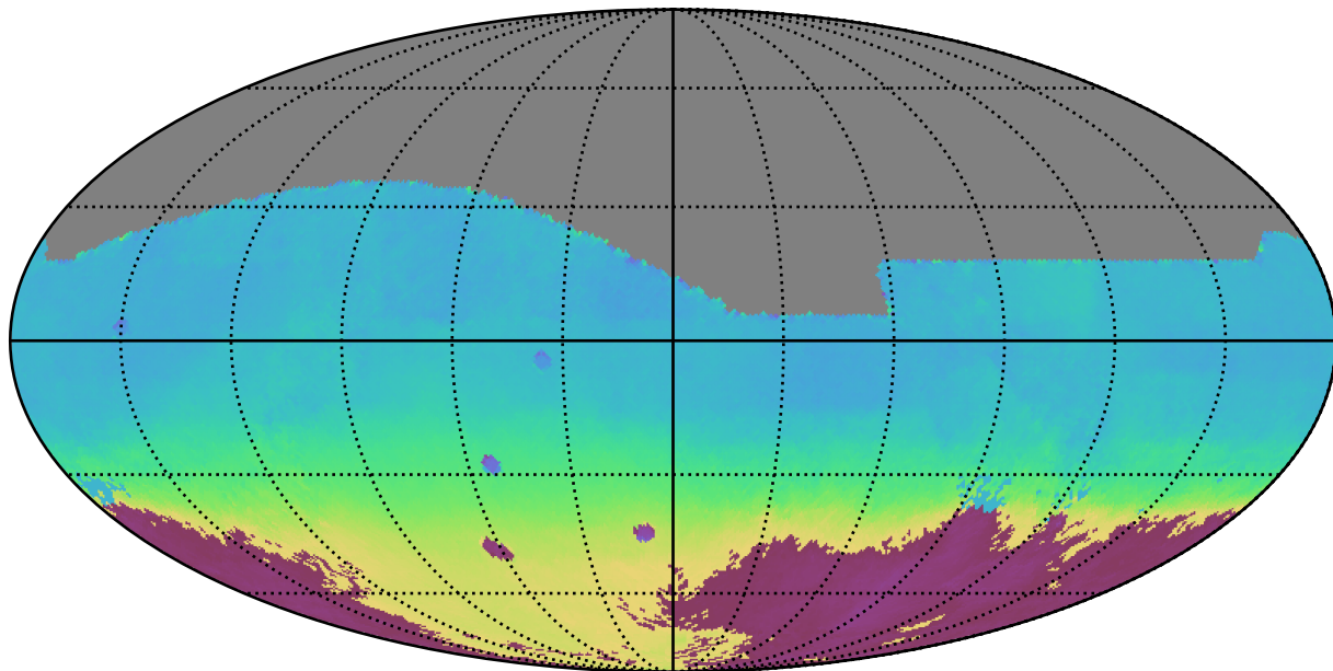
baseline_v2.1_10yrs All sky all bands: AngleMean rotSkyPos
