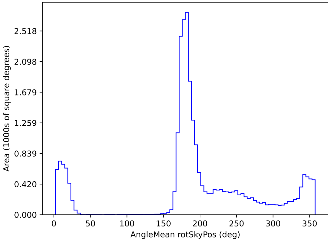
baseline_v2.1_10yrs All sky all bands: AngleMean rotSkyPos
