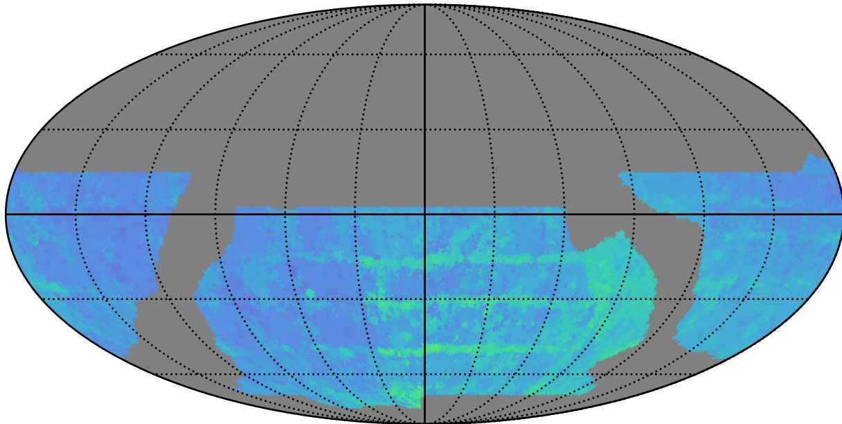
baseline_v2.1_10yrs WFD z band: 80thPercentile Season Length
