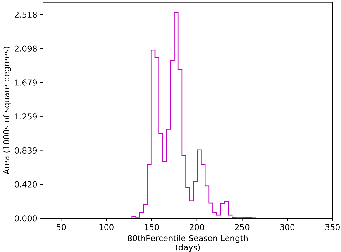
baseline_v2.1_10yrs WFD z band: 80thPercentile Season Length
