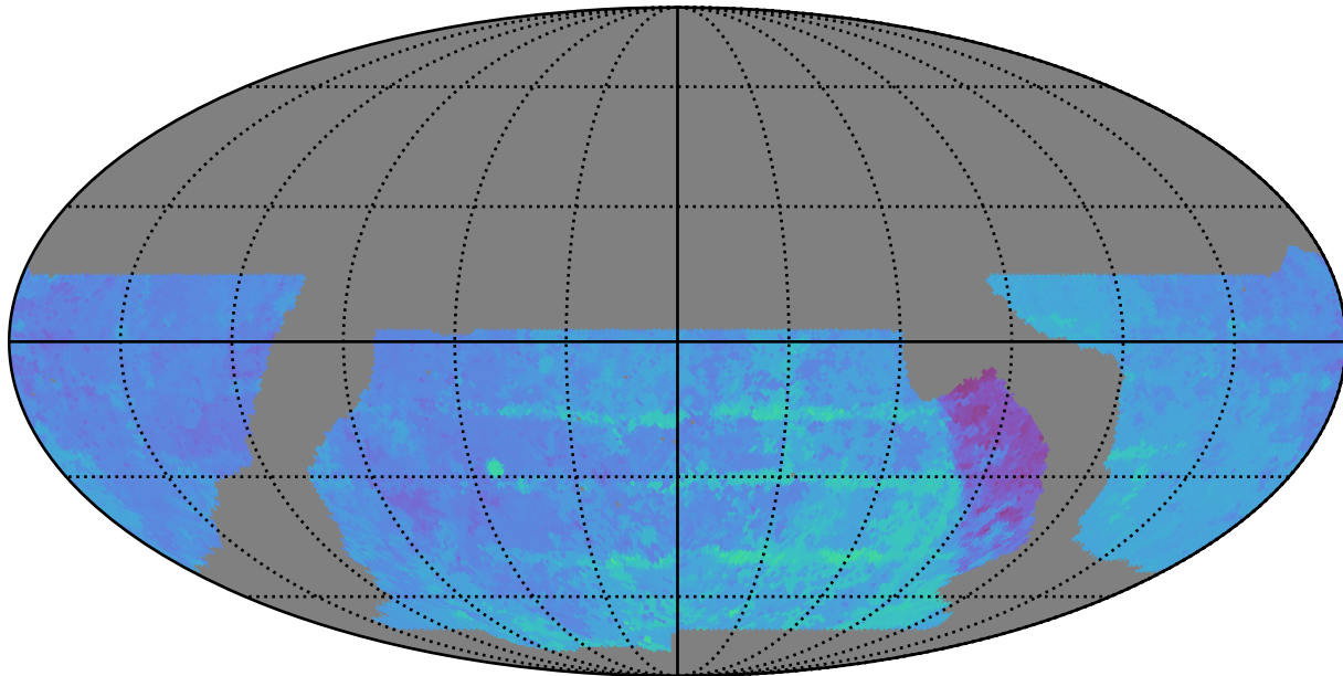
baseline_v2.1_10yrs WFD y band: 80thPercentile Season Length
