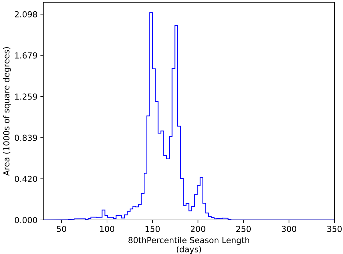
baseline_v2.1_10yrs WFD y band: 80thPercentile Season Length
