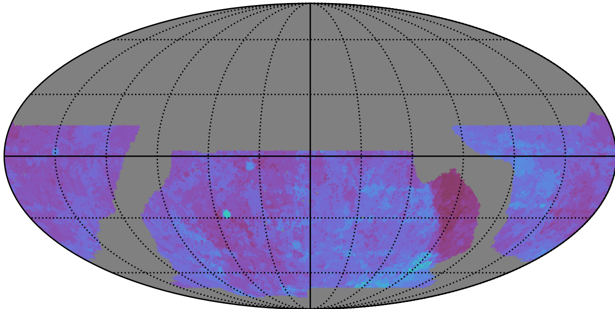
baseline_v2.1_10yrs WFD u band: 80thPercentile Season Length
