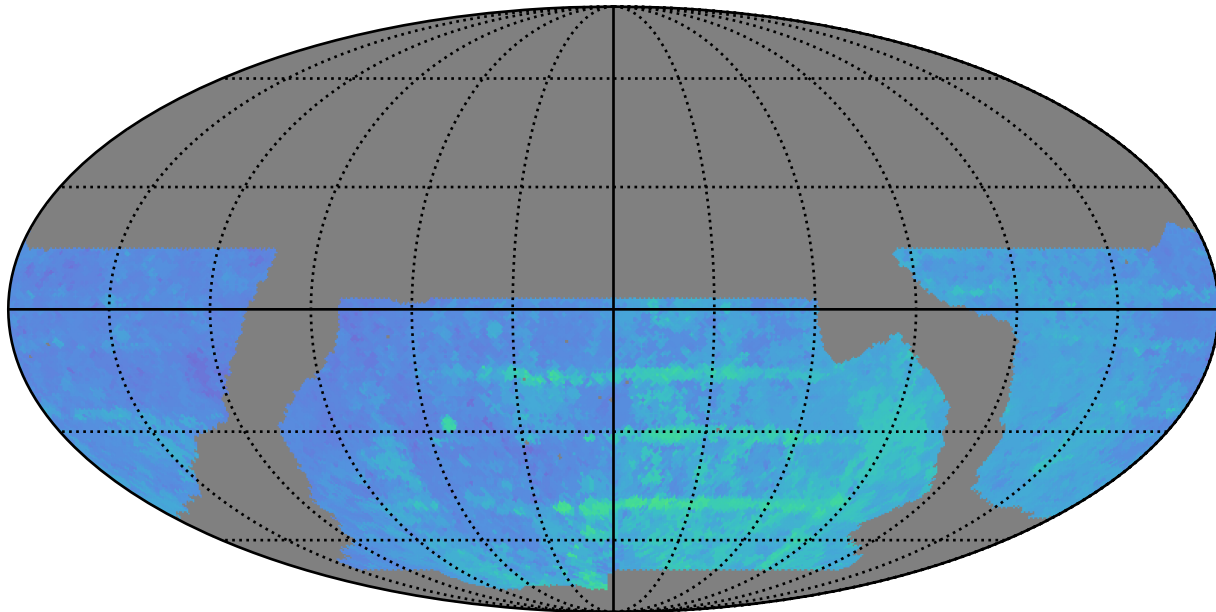
baseline_v2.1_10yrs WFD r band: 80thPercentile Season Length
