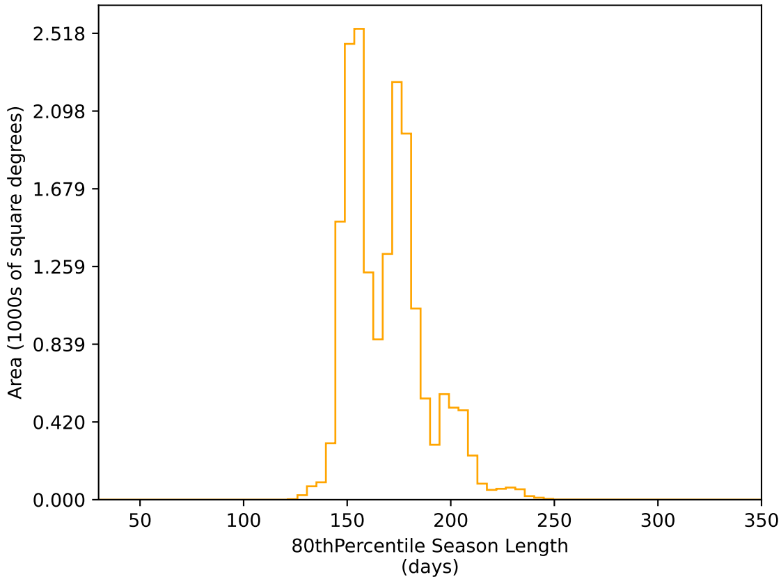
baseline_v2.1_10yrs WFD r band: 80thPercentile Season Length
