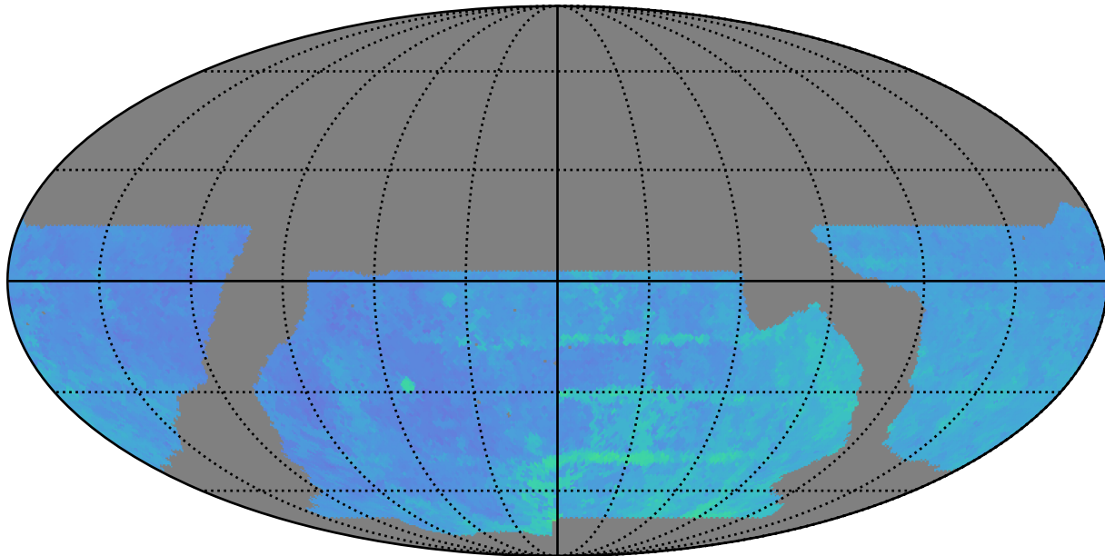
baseline_v2.1_10yrs WFD i band: 80thPercentile Season Length
