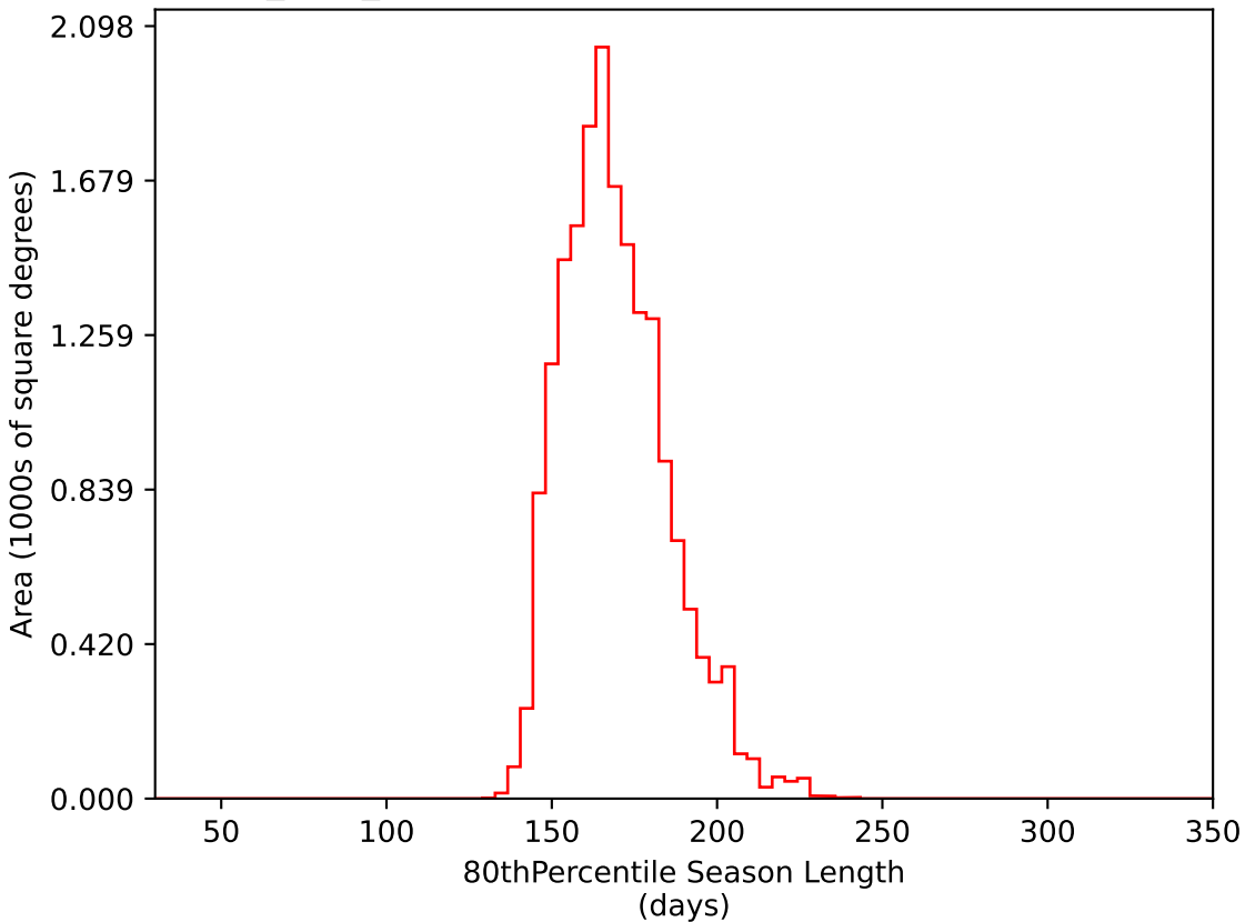
baseline_v2.1_10yrs WFD i band: 80thPercentile Season Length
